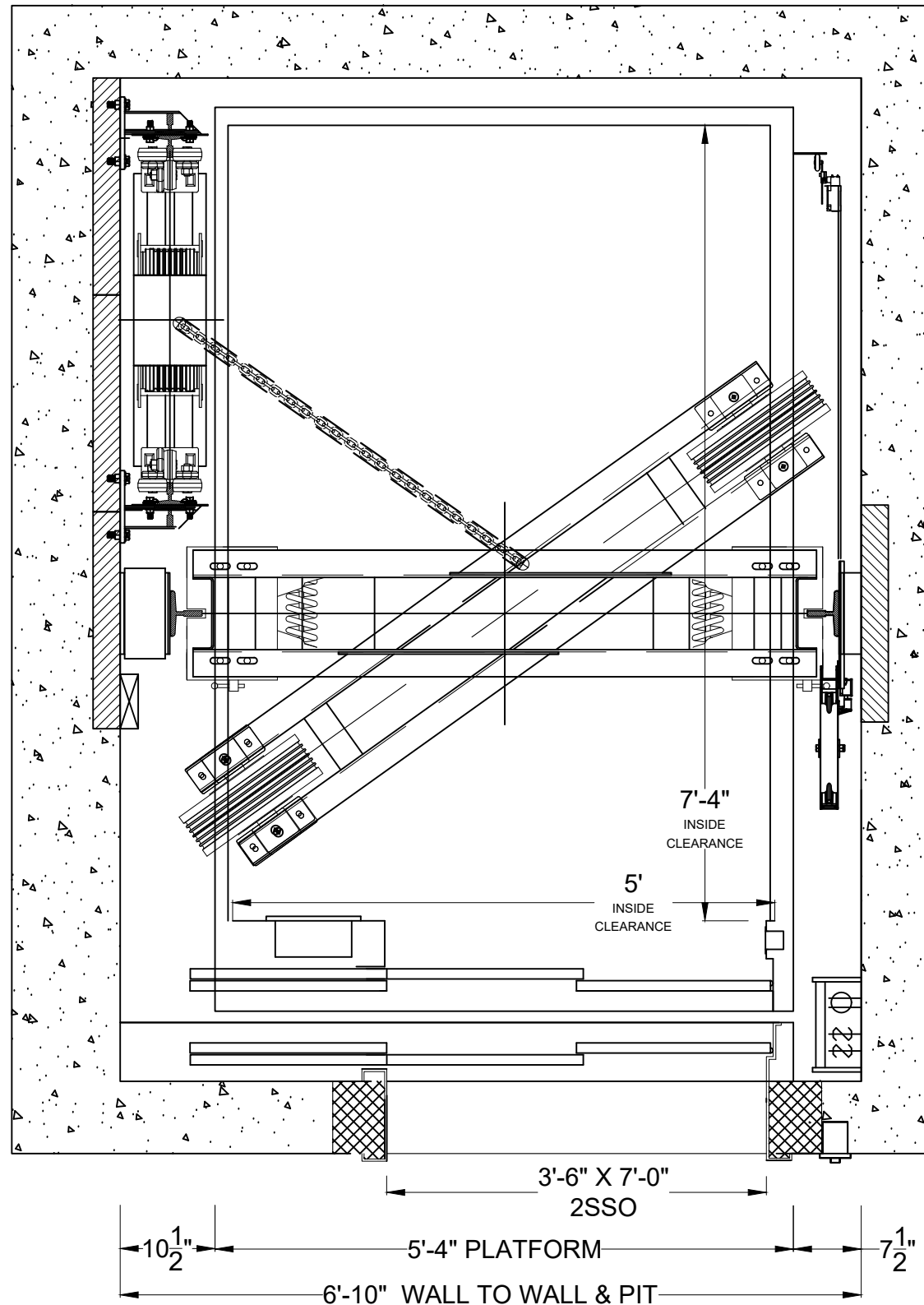
MRL 3,500 SERVICE FRONT ONLY BLDG SUPPORTED DIMENSIONS SHOWN ARE FOR SEISMIC ZONE 0
